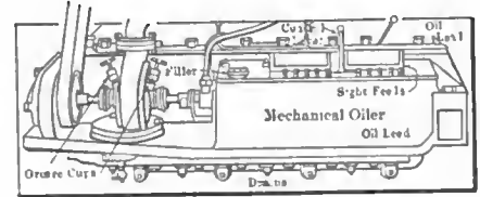
Fig. 3—The mechanical oiler of the Amplex and indication of oil distribution
